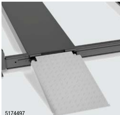
5174497 Aluminum Approach Ramps Width - 19.75" / Length - 36.75"
